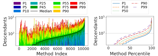
(a) Descendants sorted in increasing order (b) CDF
