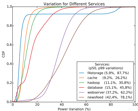
Figure 6. The measured power variations for several services in Facebook at the server level. The default time window is 60 s. For convenience, we also show the median (50 th percentile, or p50) and p99 power variation values for each case.
